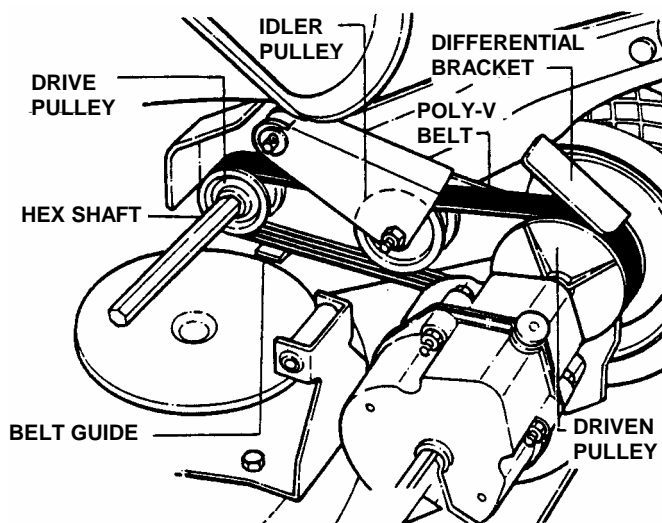
ROUTING OF POLY-V BELT FIGURE 4.17
