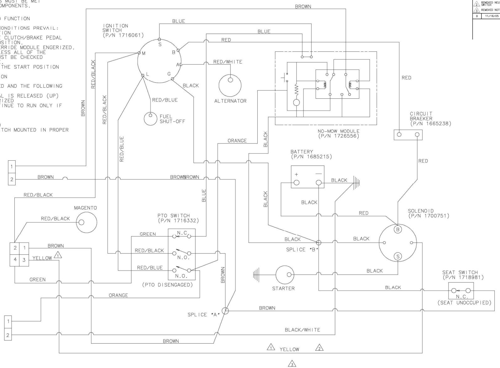
WIRING HARNESS 1726654
